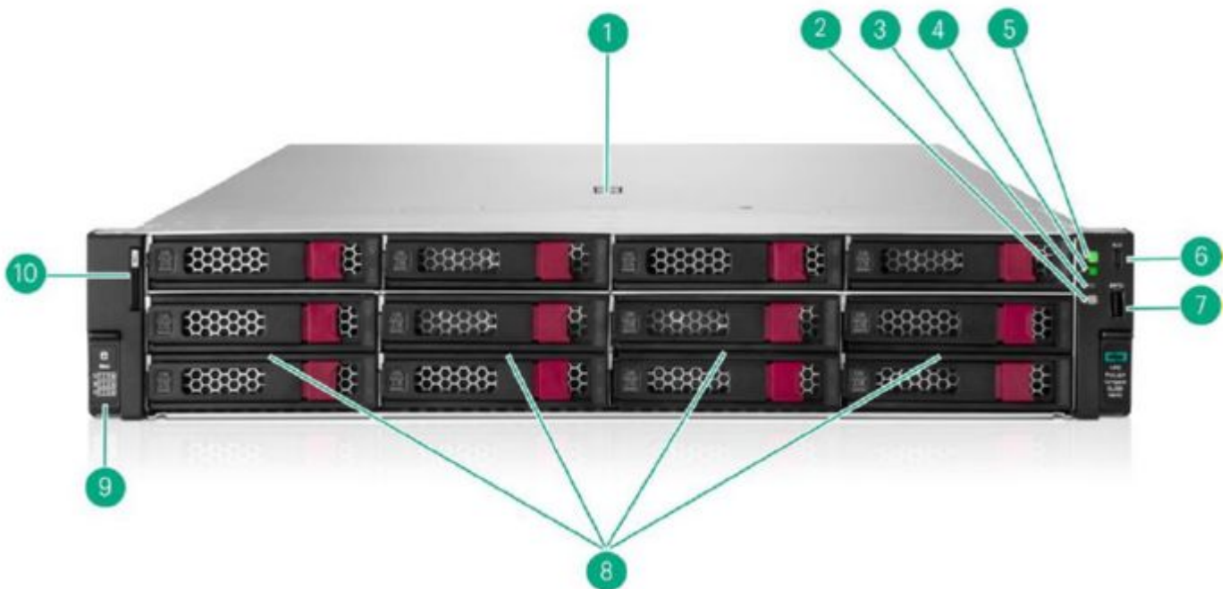
Front View - 12 LFF CTO Server
