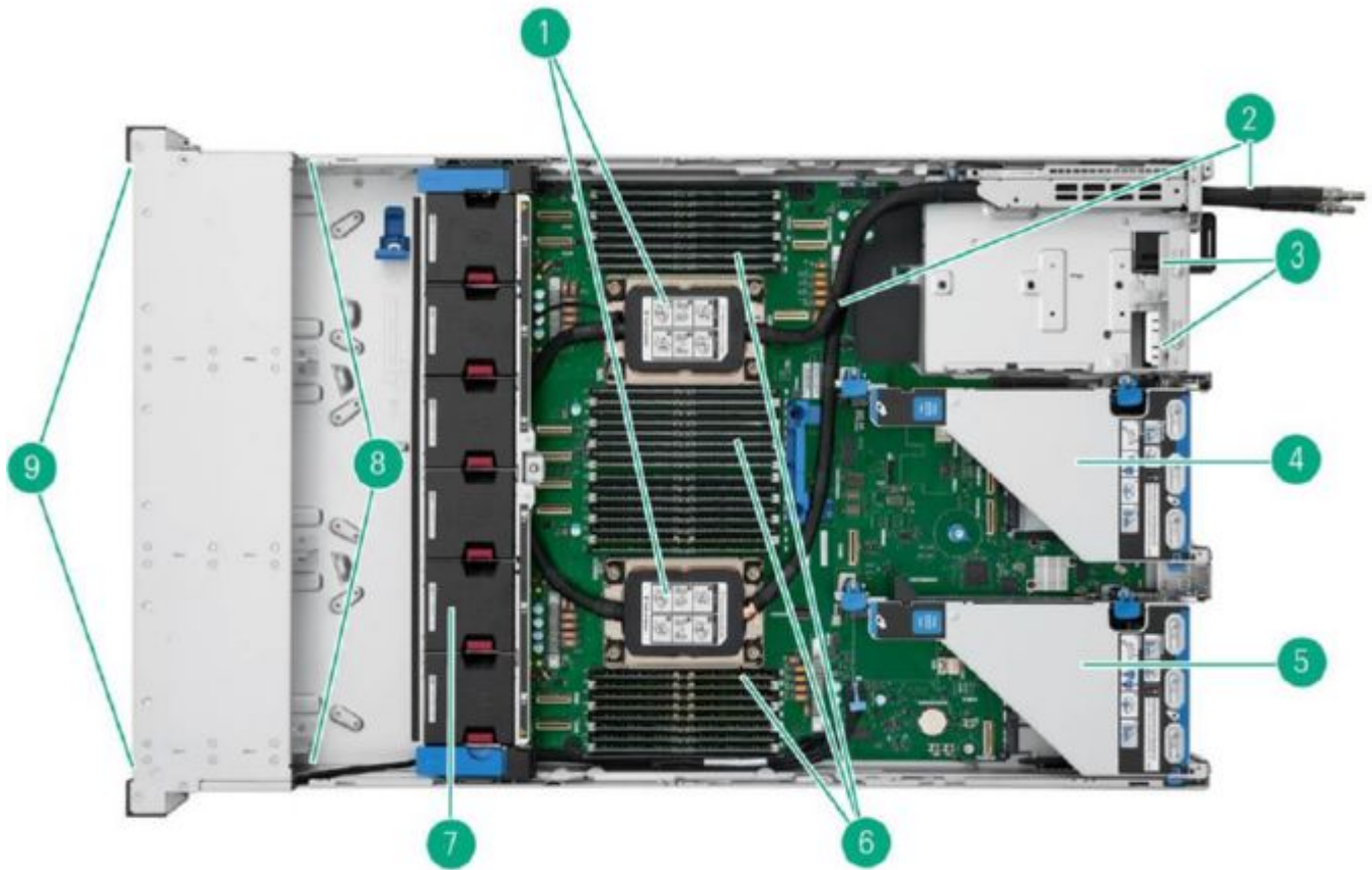
Internal View 12LFF Chassis - Direct Liquid Cooling
