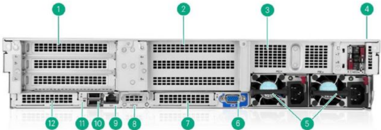
Rear View - DL380 Gen12 Air Cooled
