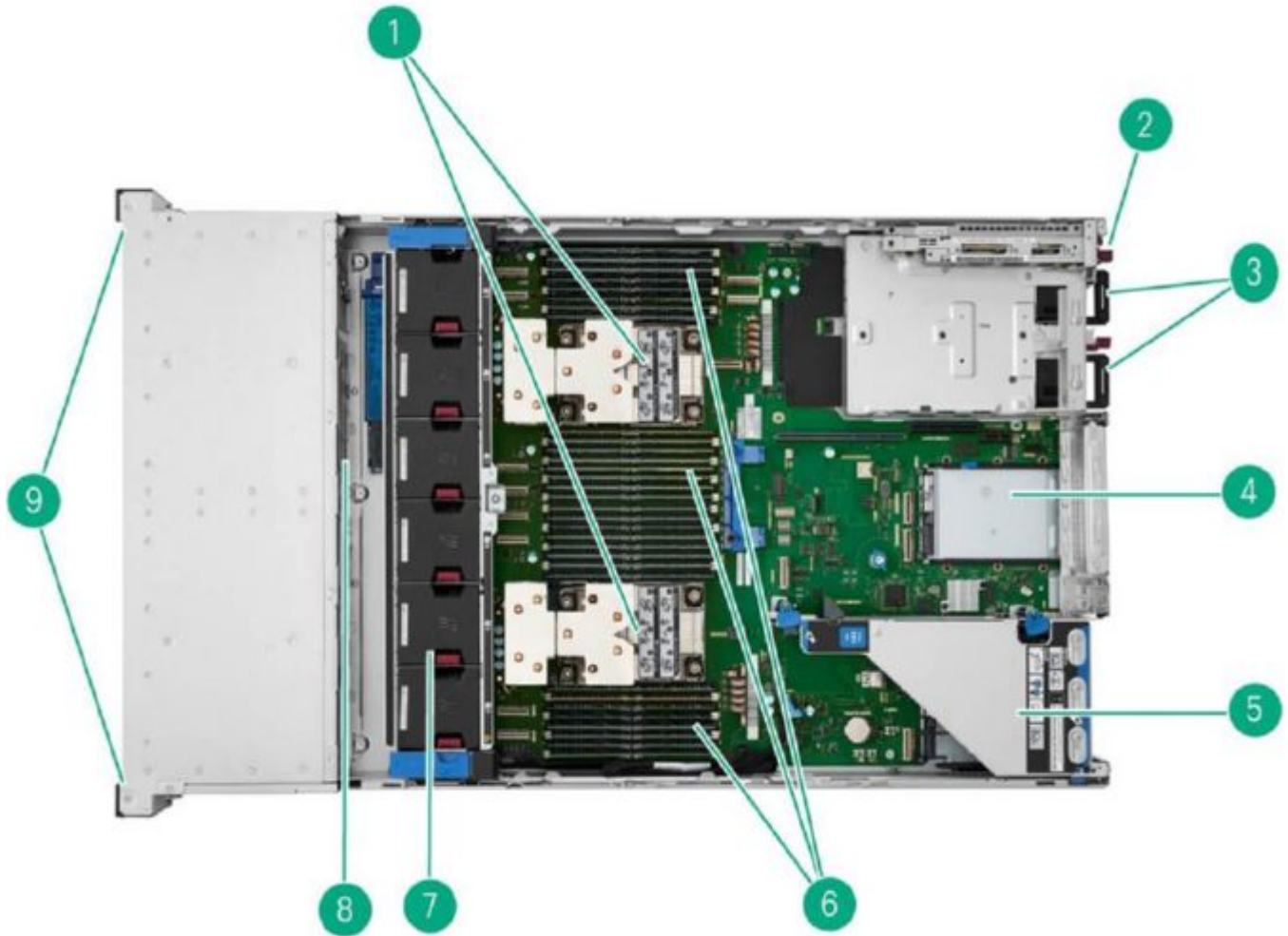
Internal View SFF chassis- Air Cooled
